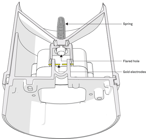
Figure 9 Rain gauge
